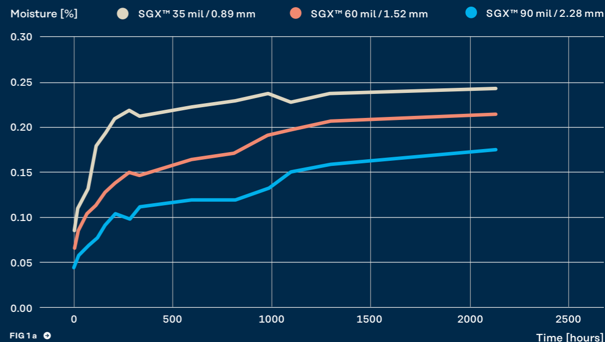
SentryGlas® Xtra™ moisture uptake at 50% RH
