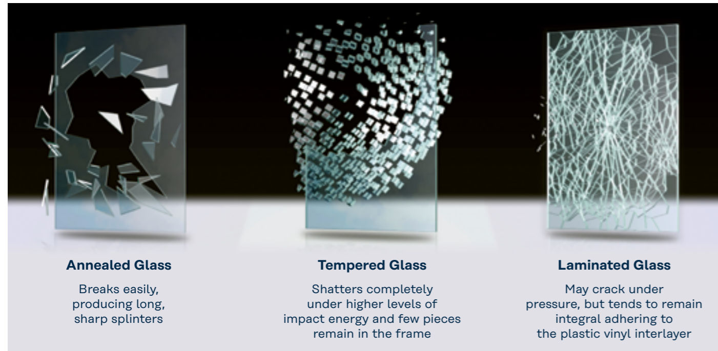
• Comparison fracturing of annealed, tempered (or heat-strengthened) glass vs. laminated glass made of annealed glass
