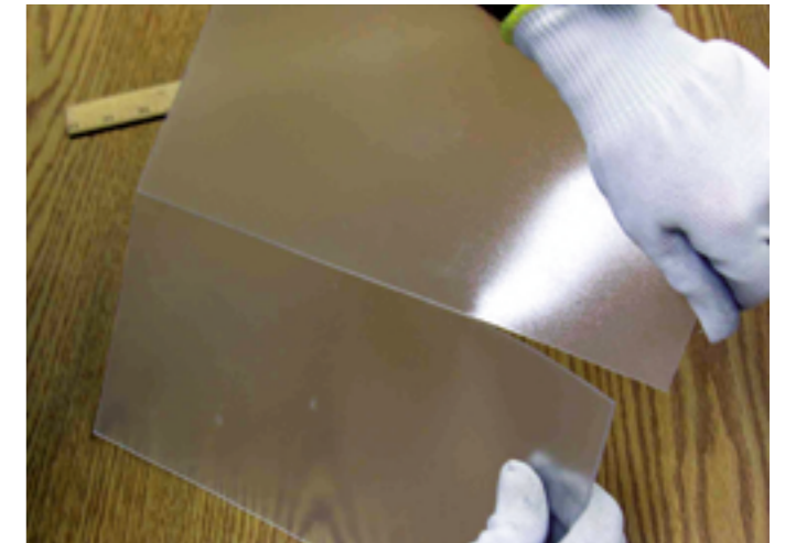
FIG 10 • Cutting SentryGlas®: Tear along scored pattern
