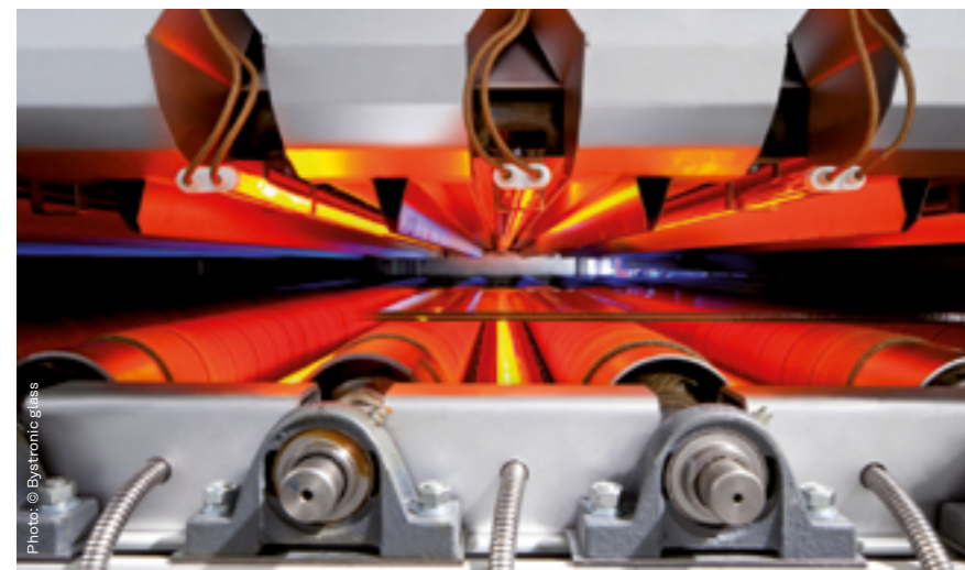
• IR heaters in nip roll oven
