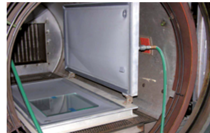
FIG 21 • Clamshell assembly (reusable)
