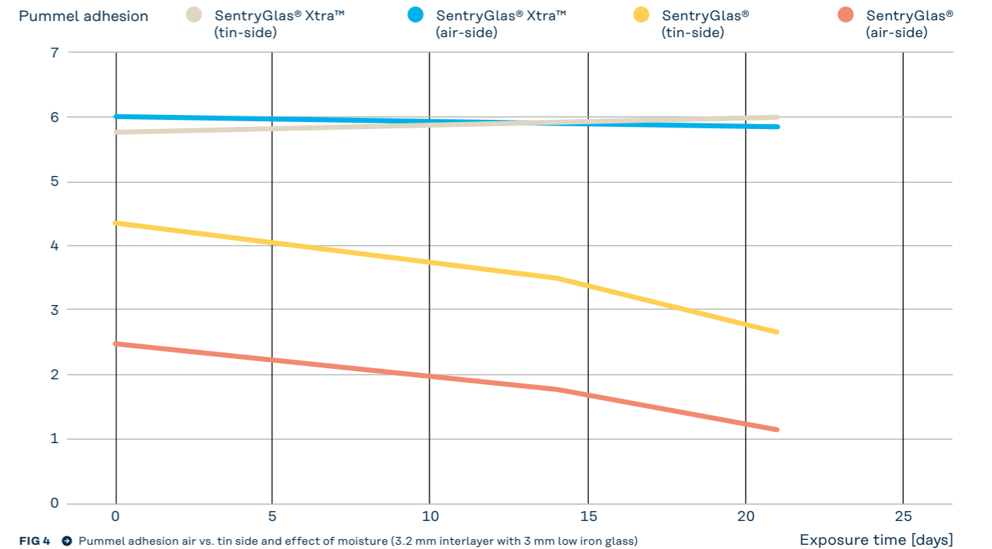
FIG 4 Pummel adhesion air vs. tin side and effect of moisture (3.2 mm interlayer with 3 mm low iron glass)
