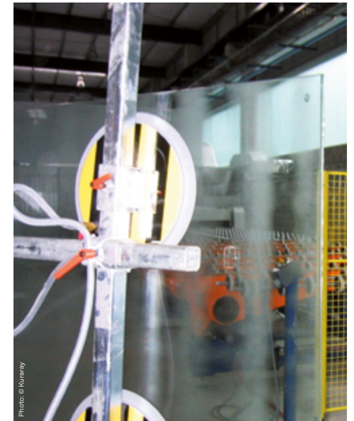
Photo: © Kuraray Laminated tempered glass nip roll result
