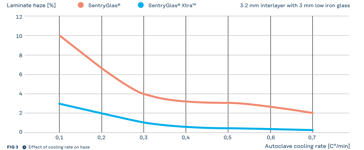
FIG 3 Effect of cooling rate on haze
