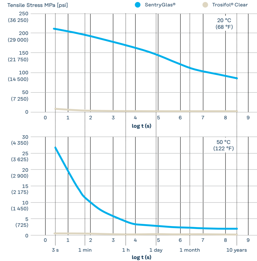
FIG 4 • The stiffness behavior of SentryGlas® at increased temperatures also shows improvements compared to PVB.
