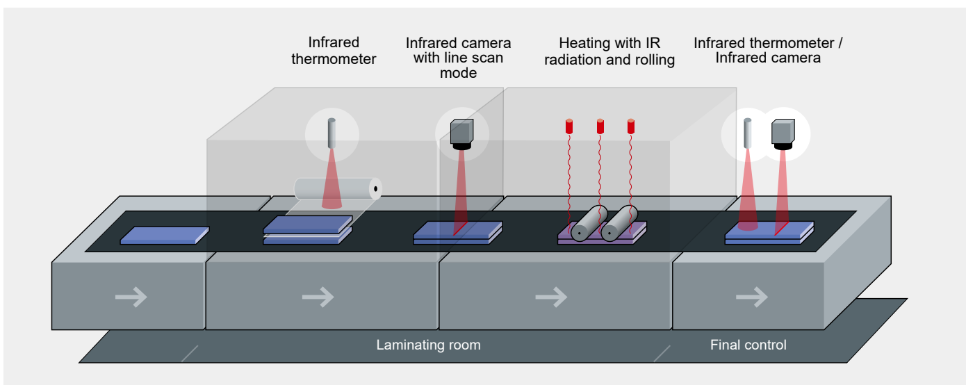
Measurement areas at LSG production
