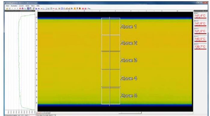
Thermal image of the endless float glass during cooling process created by an infrared camera operating in line scan mode
