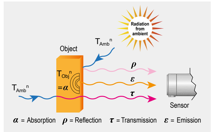
Compensating ambient influences
