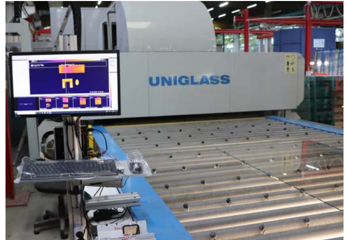
Temperature monitoring of glass sheets in a tempering machine
